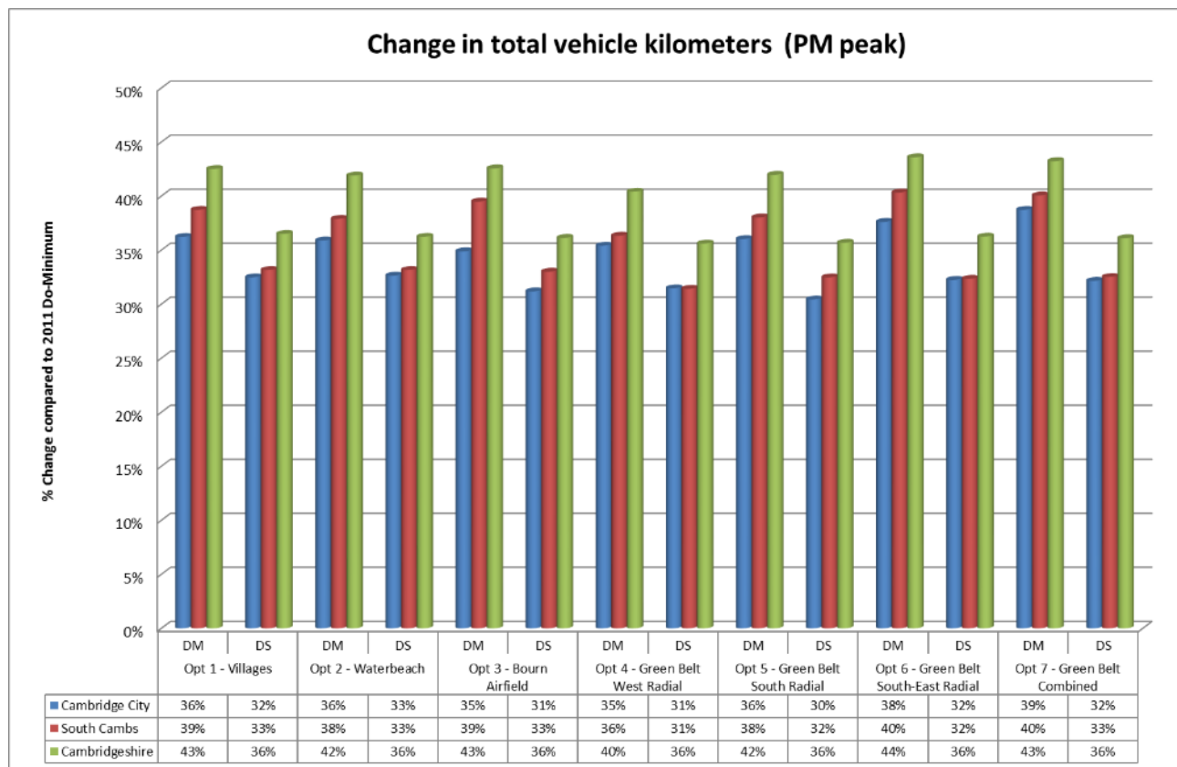
Figure 5-6 Change in total vehicle kilometres (PM peak)
